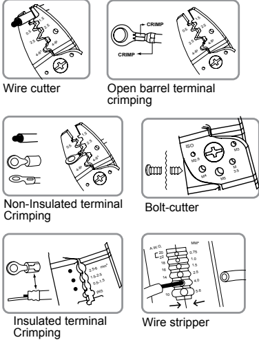
6721-10 Professional Crimping Tool 6721-10 9-3/4" 0.55 LBS $41.67
